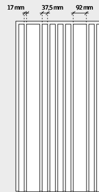
Troldtekt® line design 11, 3/9 (without grooves 3 and 9)
