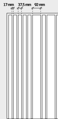
Troldtekt® line design 11, 7/10 (without grooves 7 and 10)
