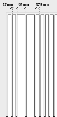
Troldtekt® line design 11, 4/6 (without grooves 4 and 6)
